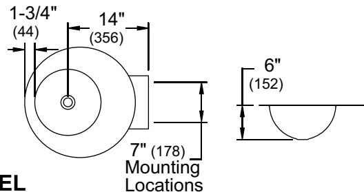
MODEL 8931-RLL-H0
