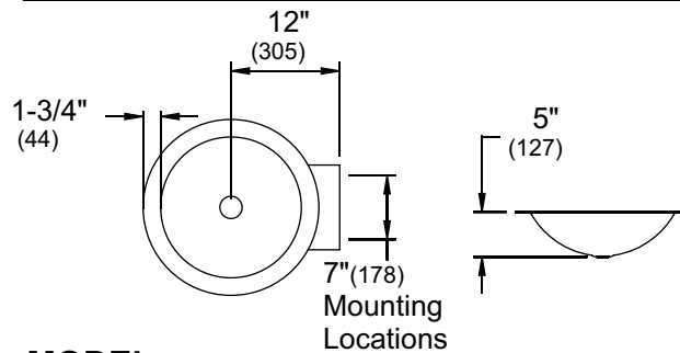
MODEL 8931-RLL-H0
